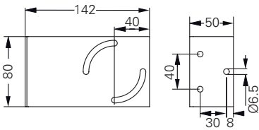
Mounting bracket
