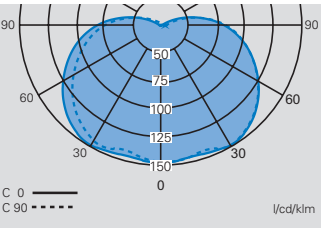
Polar curve dKLK 23 LED
