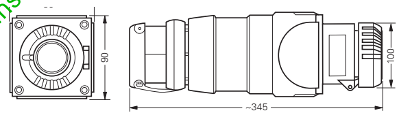
Coupler 5-pole
