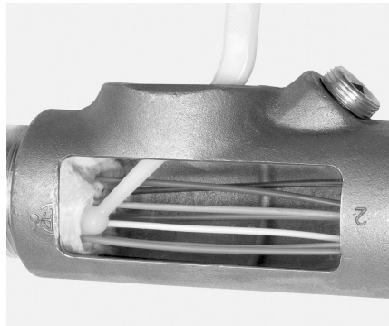
With one of the packing tools, packing fiber in between and around electrical conductors is effortless
