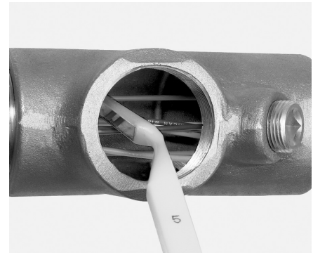
The mirrored tool allows for proper inspection of the fiber dam in difficult to see areas
